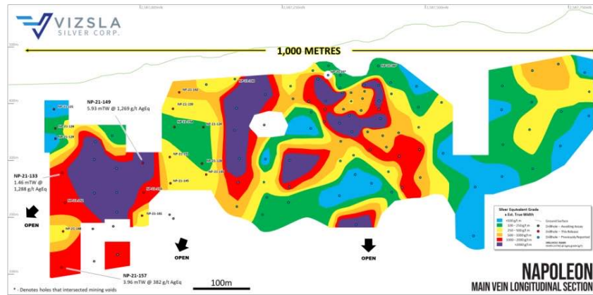
Longitudinal mining section of the Napoleon vein as reported on Vizsla Silver press release dated September 02, 2021
